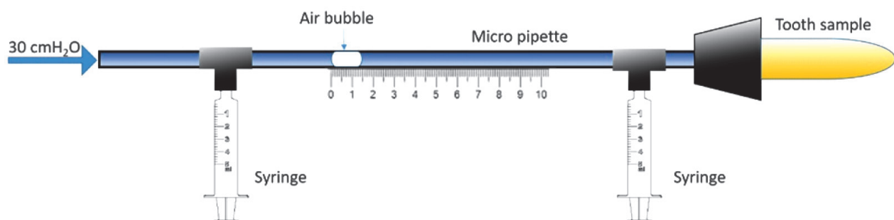
Figure 1 Fluid filtration device for leakage determination.
