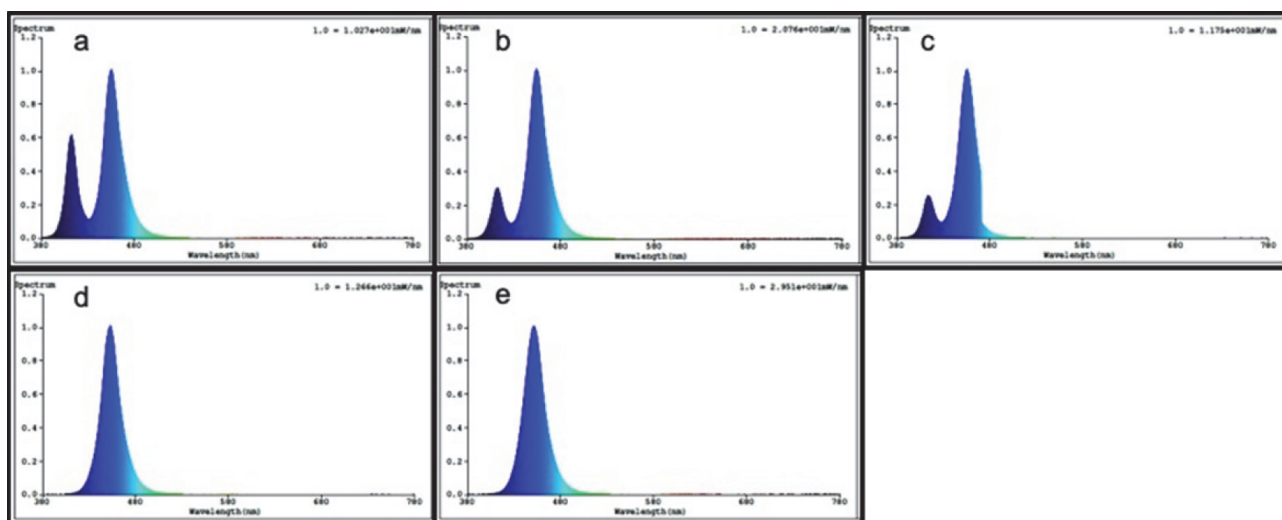
Figure 3 Spectral emission of the different LED curing units used in this study. (a: Bluephase G2 High Intensity, b: Bluephase G2 Low Intensity, c: Bluephase Style, d: Demi Plus, e: Elipar S10).
