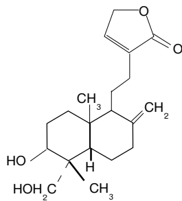
Deoxyandrographolide
