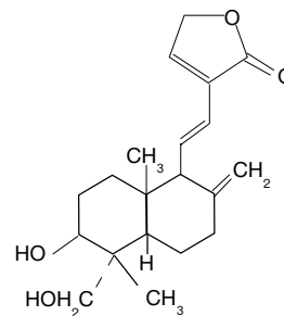
Deoxy-didehydroandrographolide
