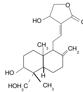
Andrographolide
