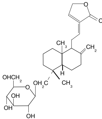
Neoandrographolide
