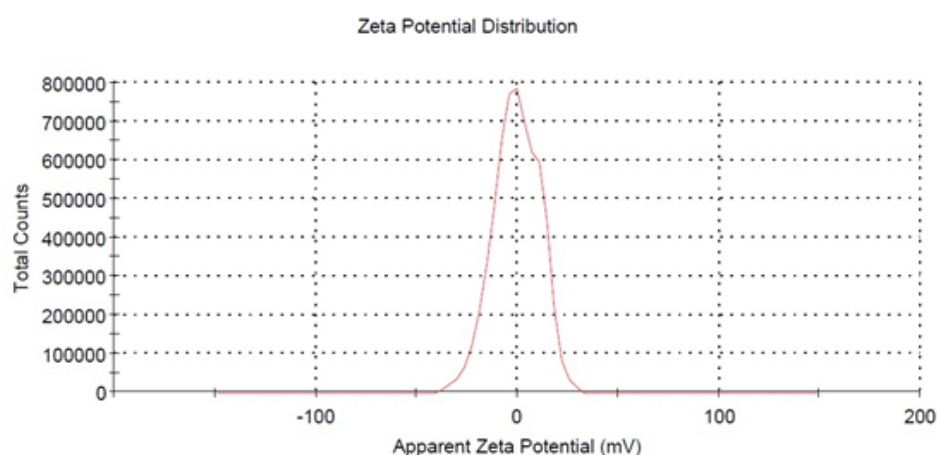
Figure 4 Zeta potential graph of GM-CuNPs. The appearance of maximum peak elicited at -0.37 \pm 11.3 mV..
