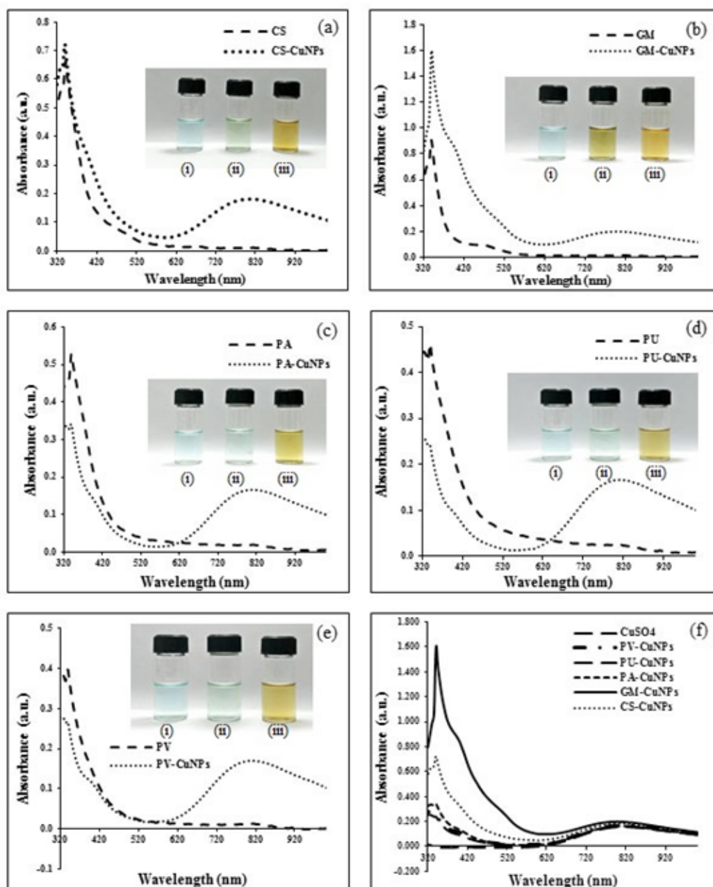
Figure 2 Ultraviolet-Visible absorption spectrum of (a) CS and CS-CuNPs (b) GM and GM-CuNPs (c) PA and PA-CuNPs (d) PU and PU-CuNPs (e) PV and PV-CuNPs and (f) \text{CuSO}_4 and all CuNPs intensity. (i) = \text{CuSO}_4 , (ii) = \text{CuSO}_4 + extract, and (iii) = extract.
