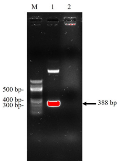
Figure 1 Amplification of ORF7 gene by RT-PCR analyzed in 1% agarose gel stained with fluorescent dye (GeneDireX, Taiwan). Lane M = 100 bp DNA marker (BioLabs, USA), Lane 1 = 388 bp PCR product, Lane 2 = negative control.
