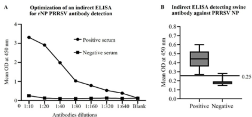
Figure 4 Indirect ELISA optimization and cutoff value evaluation. (A) The optimum concentration of rNP was tested with two-fold serial dilutions of positive and negative swine sera. (B) Detection of swine antibody against PRRSV nucleoprotein by iELISA in positive and negative sample from IDEXX PRRS X3 Ab Test. The boxplot illustrates the distribution of mean O.D. values from 15 positive and 15 negative swine sera at 0.25 cutoff value.
