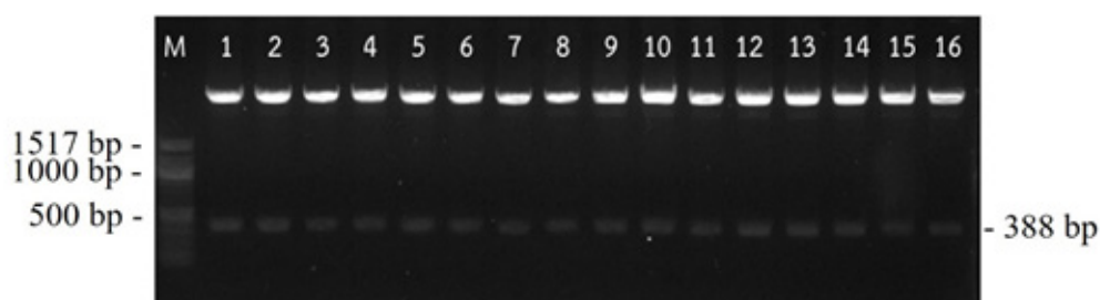
Figure 2 Restriction enzyme digestions of pGEM ® -T Easy vectors analyzed in 1% agarose gel stained with fluorescent dye (GeneDireX, Taiwan). Lane M = 100 bp DNA marker (BioLabs, USA), Lane 1-16 = 388 bp PCR product of selected positive clones.
