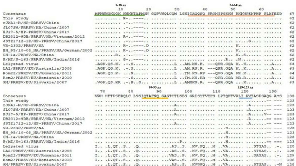
Figure 7 ClustalW Multiple alignment using BLOSUM 62 scoring Matrix with 1,000 bootstraps showed sequence alignment between our predicted rNP and 14 reference sequences of PRRSV nucleocapsid protein. The four underlines were predicted linear epitopes at 4 sites on the protein sequence ( http://tools.iedb.org/main/bcell/ ), dashes (-) represented gaps in the sequence of NP relative to its counterparts, dots (.) represented the agreement to the consensus.
