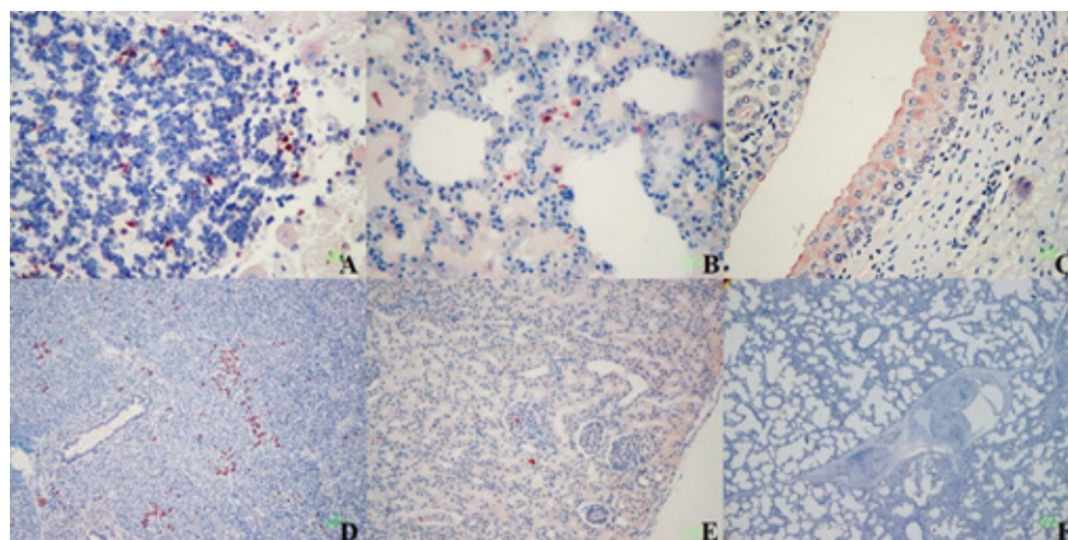
Figure 5 IHC for PRRSV in tissue stained with H&E. The red-brown color represents positive PRRSV. (A) cerebellum; (B) bronchiolar epithelium; (C) trachea; (D) salivary gland; (E) kidney; (F) lung negative control. All images were obtained at a magnification of 200x.
