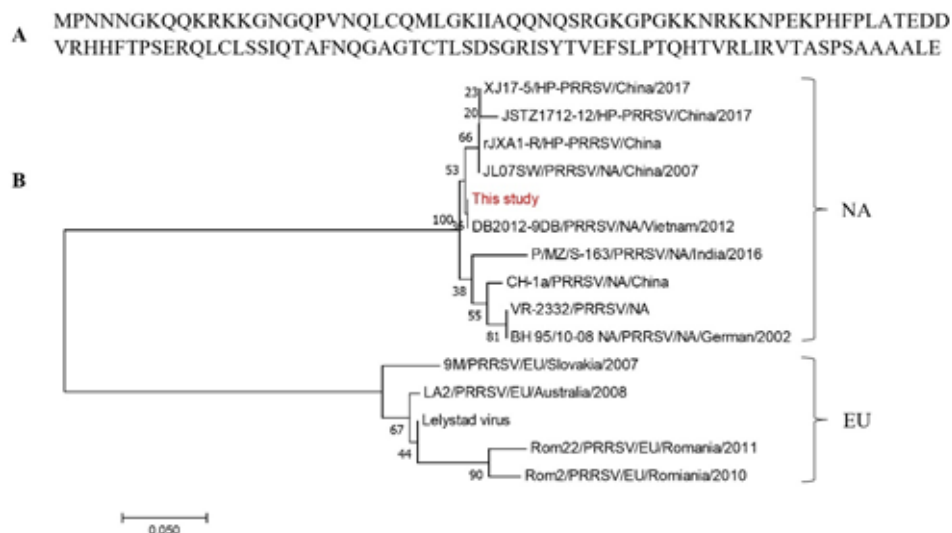
Figure 6 Analysis of amino acid sequence of the rNP. (A) Amino acid sequence of 128 aa translated by Expasy website. (B) Neighbor-Joining tree of PRRSV nucleocapsid protein. Phylogenetic analysis showed that the protein in this study (red) was nucleocapsid of PRRSV by comparing with 14 reference sequences.
