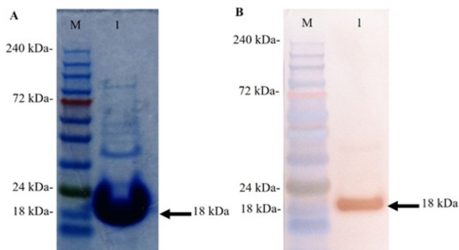
Figure 3 (A) SDS PAGE and (B) Western blot of the rNP-His-tag expressed in E. coli BL21. Lane M = protein marker (Bio-Helix, Taiwan); Lane 1 = purified rNP (18 kDa).
